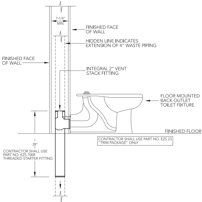
RIGHT HAND FITTING - LEFT SIDE ELEVATION
