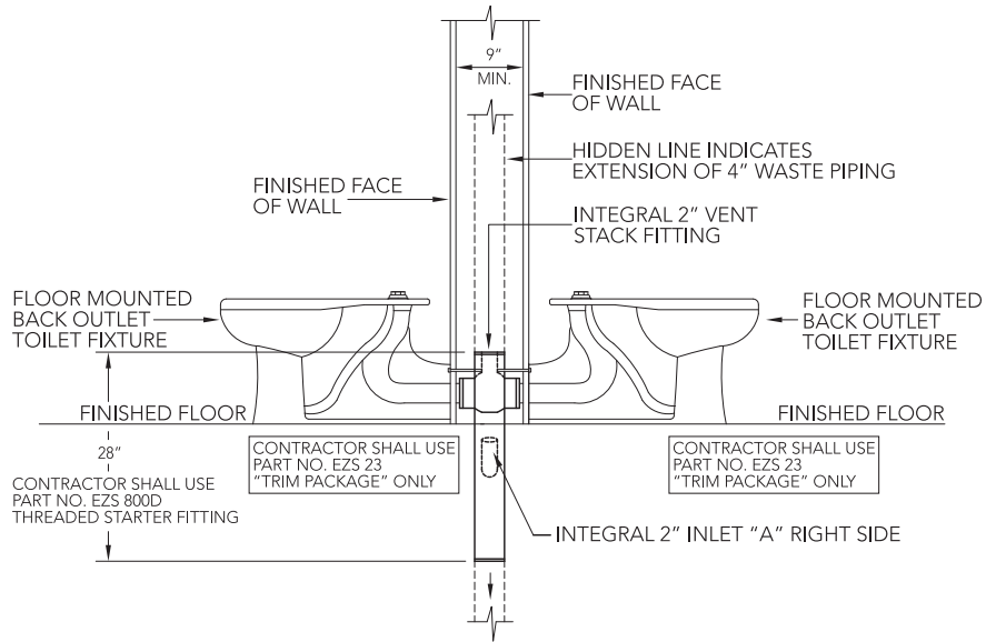
DOUBLE FITTING - LEFT SIDE ELEVATION
