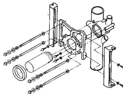
EZS 22 and EZS 24 Assemblies Illustrated
