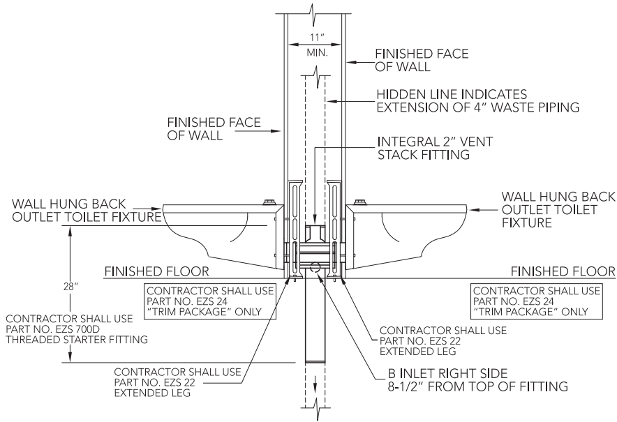
DOUBLE FITTING - LEFT SIDE ELEVATION
