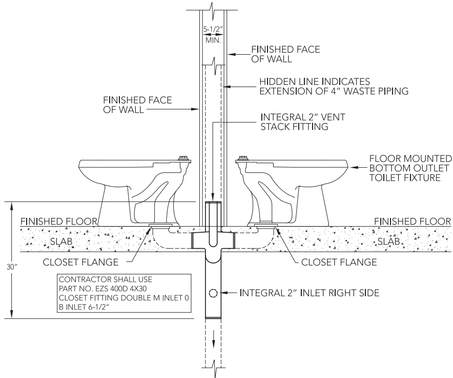
DOUBLE FITTING IN-SLAB - LEFT SIDE ELEVATION
