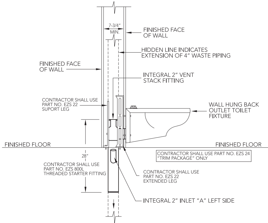
LEFT HAND FITTING - LEFT SIDE ELEVATION
